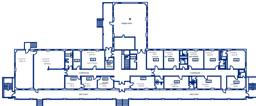
BLDG 205, 1st FLOOR PLAN
