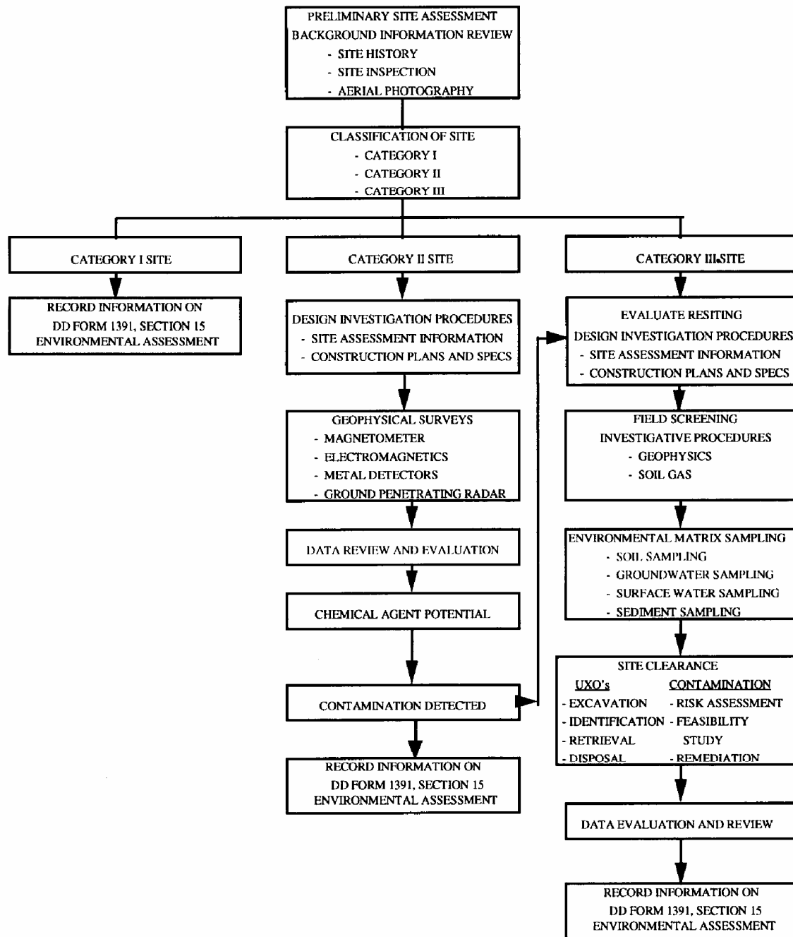
Figure 15-1. Conceptual elements of site investigation and clearance
