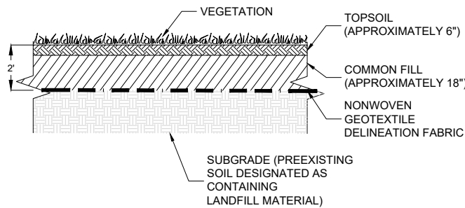
VEGETATIVE CAP (TYPICAL, NOT TO SCALE)
